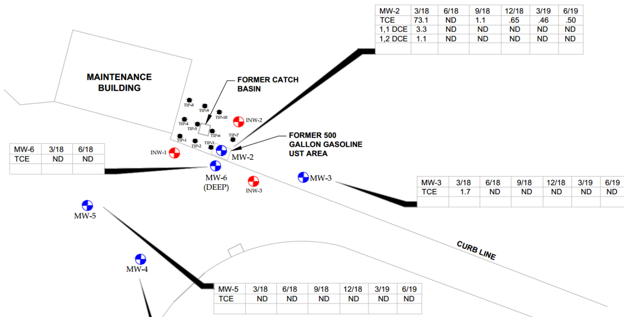
Figure 2. CVOC Concentrations in Groundwater Reductions
